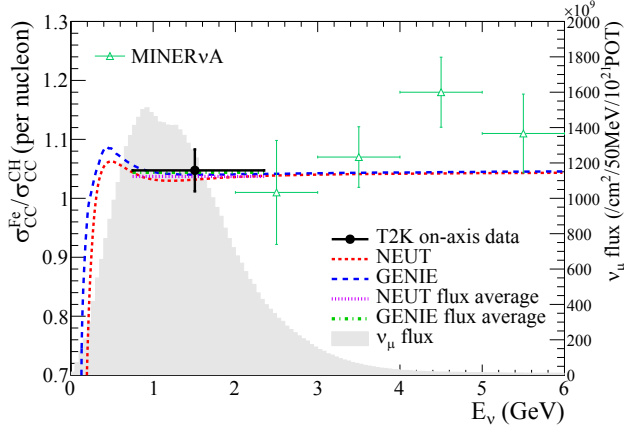
FIG. 21. The inclusive \nu_\mu charged current cross section ratio on Fe to CH with predictions by NEUT and GENIE. The isoscalar corrections are not applied to our data or predictions. Our data point is placed at the flux mean energy. The vertical error bar represents the total (statistical and systematic) uncertainty, and the horizontal bar represents 68% of the flux at each side of the mean energy. The MINERνA result is also plotted [16].
