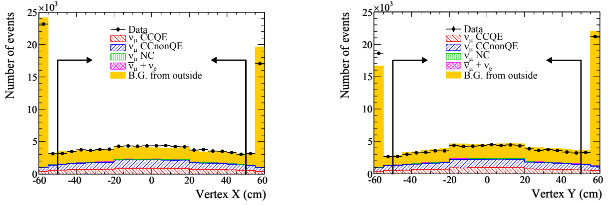
FIG. 12. Vertex X and Y distributions for the Proton Module after applying the veto cut. A volume within \pm 50 cm in the X and Y directions from the module center is defined as fiducial volume (FV). Most of the background events which pass the FV cut in one direction (X or Y) are actually rejected by the FV cut in the other direction (Y or X).
