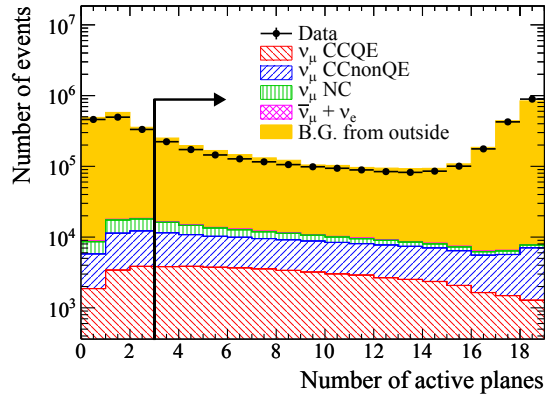
FIG. 8. Number of active planes for the Proton Module. Events with more than two active planes are selected. The background events from the walls of the detector hall is normalized with beam induced muon backgrounds, as described in Sec. IV A 9
