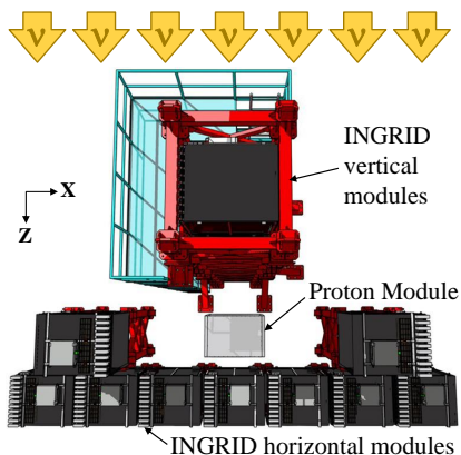
FIG. 4. The position of the Proton Module viewed from above.
