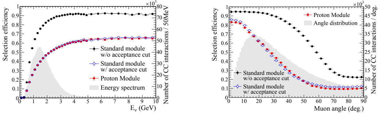
FIG. 17. Event selection efficiency of CC interactions for the standard module and the Proton Module as a function of true neutrino energy (left) and true muon scattering angle (right). The energy spectrum and angle distribution of the CC interactions in the standard module are overlaid.
