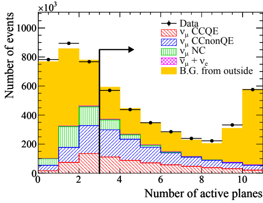
FIG. 14. Number of active planes for the standard module. Events with more than two active planes are selected.
