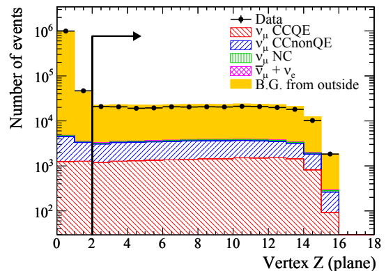
FIG. 11. Vertex Z distribution for the Proton Module before applying the veto and fiducial volume cuts.
