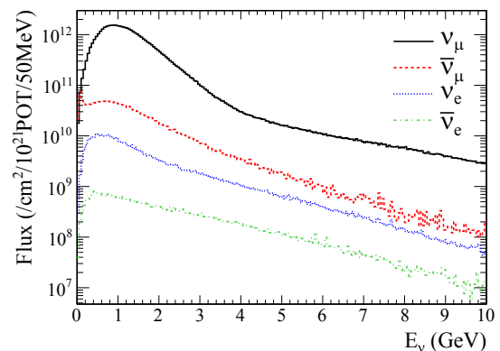
FIG. 6. Neutrino energy spectrum for each neutrino species at the central module predicted by JNUBEAM.
