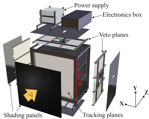
FIG. 5. Exploded view of the Proton Module.
