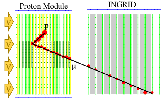
FIG. 9. MC event display of a charged current neutrino event in the Proton Module. Red circles and black lines represent observed hits and reconstructed tracks, respectively. Areas of red circles correspond to light yields.
