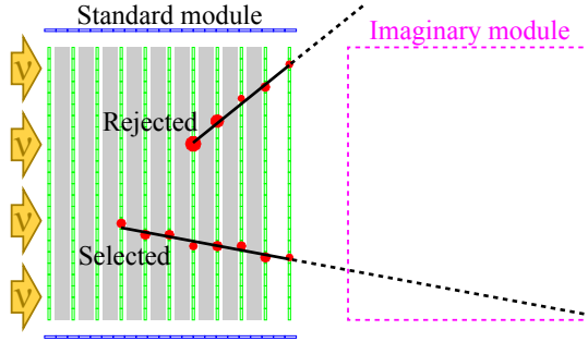
FIG. 18. MC event display of a selected event and a rejected event by the acceptance cut.
