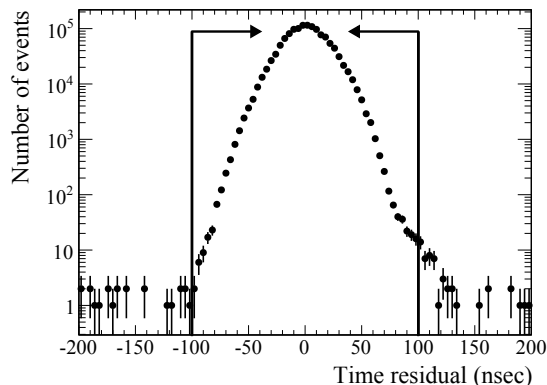
FIG. 10. Time difference between the measured event timing and the expected neutrino event timing for the Proton Module. Events within \pm 100 nsec are selected.
