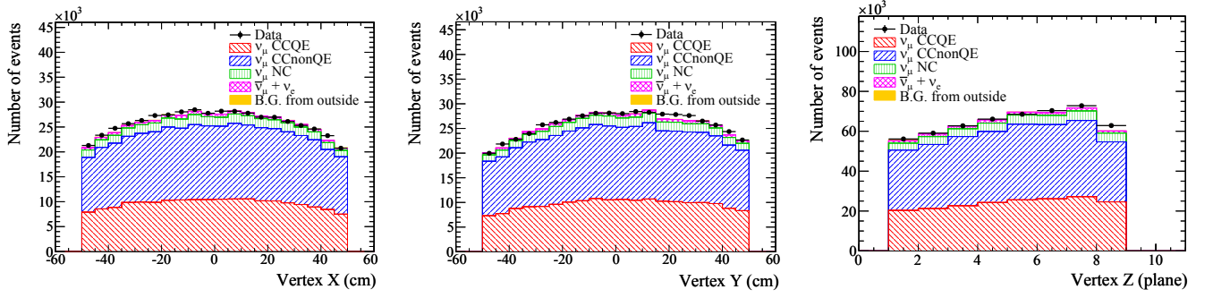
FIG. 19. Vertex X, Y and Z distributions for the standard module following event selection.
