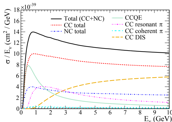
FIG. 7. Neutrino-nucleus cross sections per nucleon of carbon nucleus divided by the neutrino energy predicted by NEUT.
