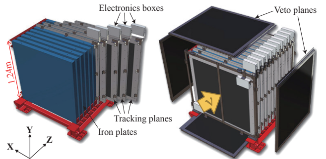
FIG. 3. Exploded view of an INGRID standard module. It consists of iron target plates and tracking scintillator planes (left), and it is surrounded by veto scintillator planes (right).
