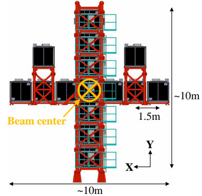
FIG. 2. Overview of the 16 INGRID standard modules viewed from beam upstream.
