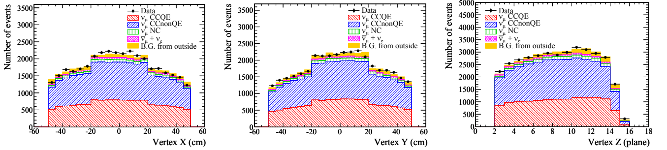
FIG. 13. Vertex X, Y and Z distributions for the Proton Module following event selection. There are jumps at X or Y = \pm 20 cm because the Proton Module uses thicker scintillators in the inner region ( -20 cm \sim +20 cm).
