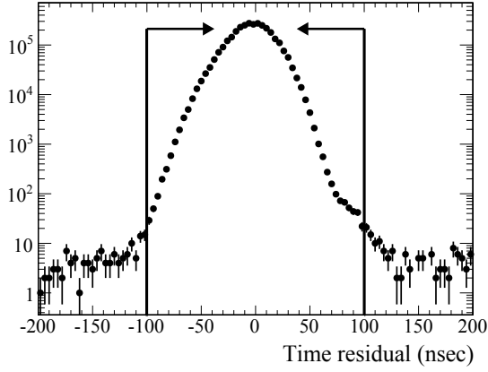
FIG. 15. Time difference between the measured event timing and expected neutrino event timing for the standard module. Events within \pm 100 nsec are selected.
