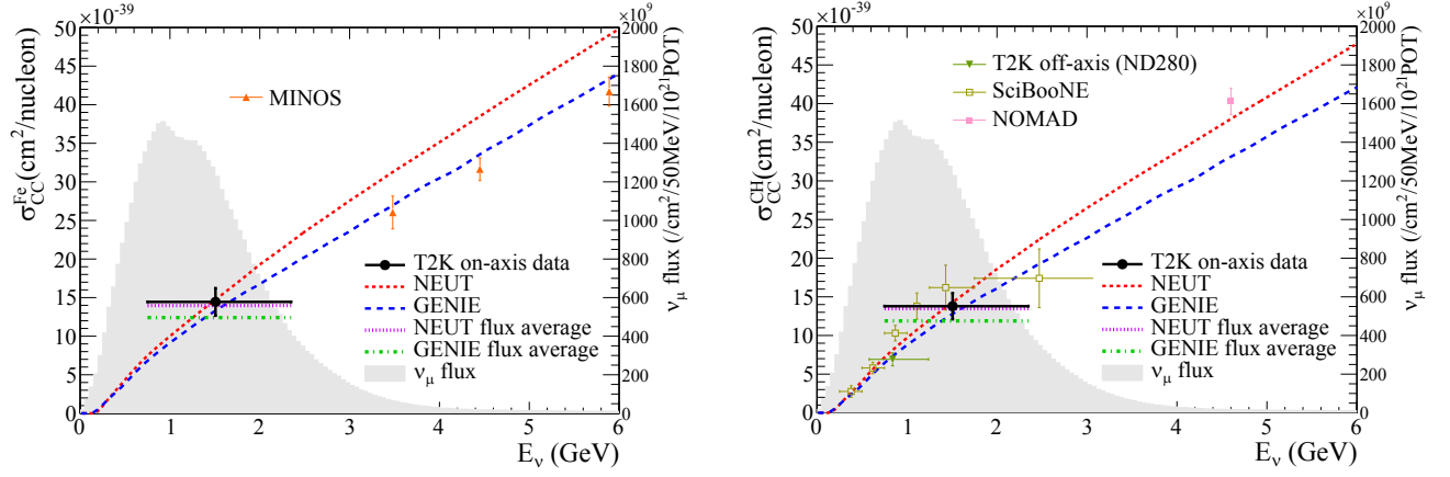
FIG. 20. The inclusive \nu_\mu charged current cross section on Fe (left) and that on CH (right) with predictions by NEUT and GENIE. The isoscalar corrections are not applied to our data or predictions. Our data point is placed at the flux mean energy. The vertical error bar represents the total (statistical and systematic) uncertainty, and the horizontal bar represents 68% of the flux at each side of the mean energy. The MINOS, T2K ND280, SciBooNE and NOMAD results are also plotted [12–15]. Because the isoscalar correction is applied to the MINOS data, it is expected to be shifted by about -2\% .
