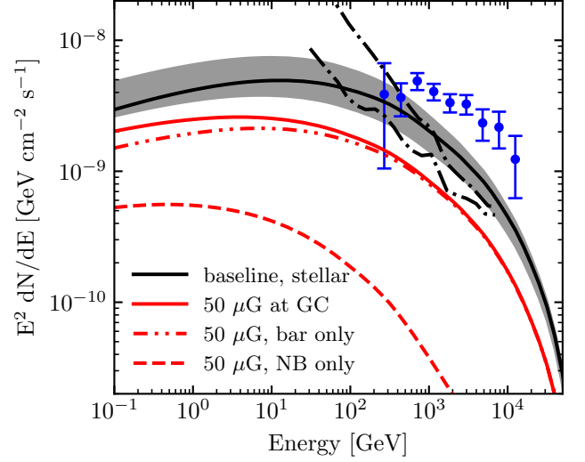
FIG. 8. IC from different magnetic field models. The baseline (black solid) adopts the original GALPROP magnetic field. The red solid introduces a 50 \mu\text{G} lower limit for the inner 400 pc region around the GC. With the presence of such a lower limit, the IC from the Galactic ridge is reduced by \sim 1/2 . Due to the higher overlap with the modified magnetic field, the IC from the NB (red dashed) is suppressed more strongly by synchrotron loss compared to the Galactic bar (red dot-dashed).
