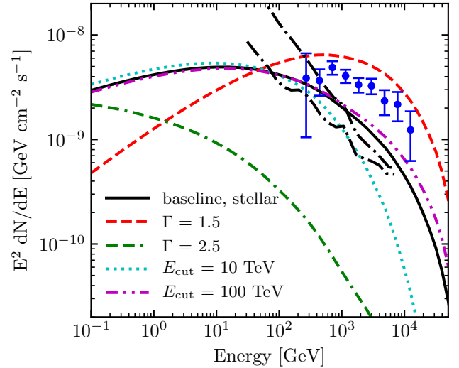
FIG. 4. IC for different E^\pm spectra as listed in Table II. H.E.S.S. data and CTA sensitivities are shown in the same way as in Fig. 3, but note the different y -axis range. Most spectra are below the H.E.S.S. measurements except for the hardest spectrum \Gamma = 1.5 with E_{\text{cut}} = 50 TeV which could be alleviated by a lower fraction of spin-down energy into relativistic e^\pm . For the soft spectrum \Gamma = 2.5 , the fluxes are below the CTA sensitivities by more than an order of magnitude.
