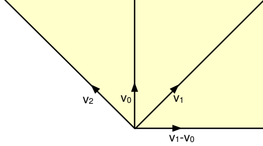
FIGURE 7. The fan \Sigma' of X' when X = K_{\mathbb{P}^1} .
