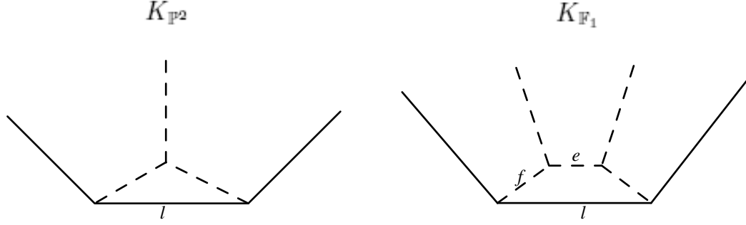
FIGURE 13. Polytope picture for K_{\mathbb{P}^2} and K_{\mathbb{F}_1} .
